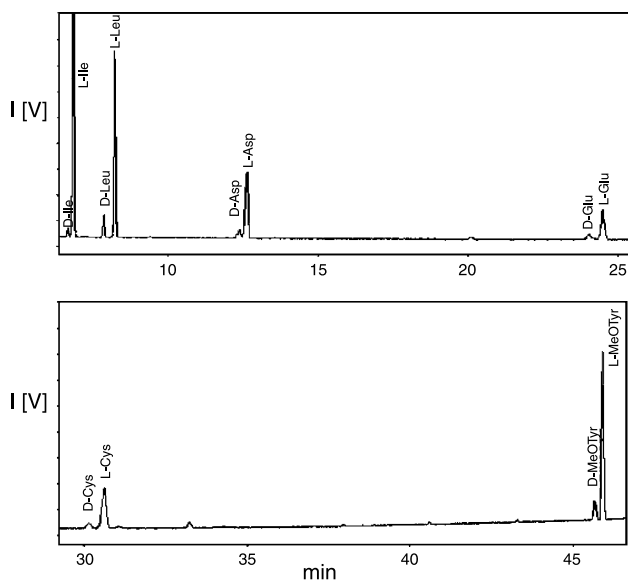
Fig. 1. GC/FID chromatograms of AA enantiomers as N,O -pentafluoropropoxycarbonyl pentafluoropropyl esters representing the ratio of D:L-AAs = 10:90 (2 nmol D-AAs:18 nmol L-AAs were derivatized) resolved on Chirasil-L-Val. For chromatographic conditions see Materials and methods
